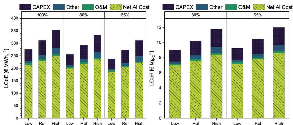
Figure 5. LCoE and LCoH estimations for the base case, i.e., 4000 FLHs and electricity price of 50 \text{ € MWh}^{-1} . (Low: lower end, Ref: reference, and High: higher end.) The \text{H}_2 kWh equivalent is estimated based on the higher heating value of 39.4 \text{ kWh kg}^{-1} .
