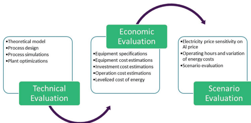
Figure 2. Methodology overview.
