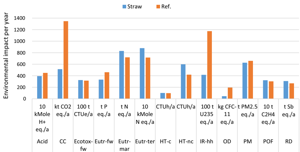
Fig. 6 Comparison of environmental impacts of the production and use of synthetic gasoline from straw (“Straw”) to fossil gasoline (“Ref.”) for the base year 2020; Acid Acidification, CC Climate Change, Ecotox-fw Ecotoxicity—freshwater, Eutr-fw Eutrophication—freshwater, Eutr-ter Eutrophication—terrestrial, HT-c Human Toxicity—cancer effects, HT-nc Human Toxicity—non-cancer effects, IR-hh Ionizing Radiation—human health, OD Ozone Depletion, PM Particulate Matter/Respiratory Inorganics, POF Photochemical Ozone Formation, RD Resource Depletion, Mineral, Fossil and Renewable
